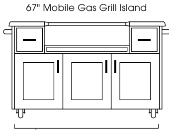
64" one-piece cabinet with 3 under-grill storage areas and locking heavy duty caster wheels
